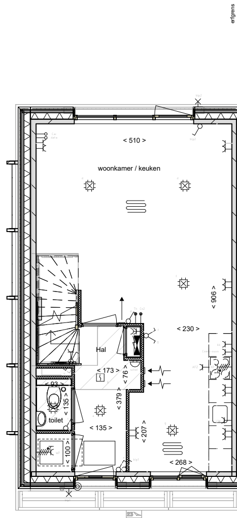
00 begane grond
